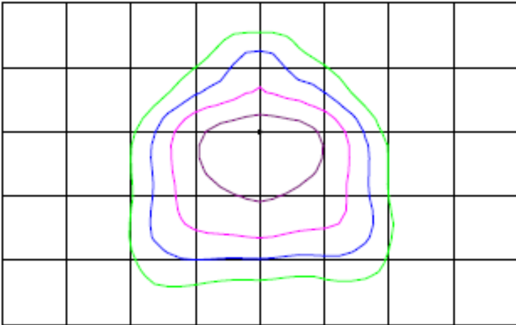
Type IV: forward throw
