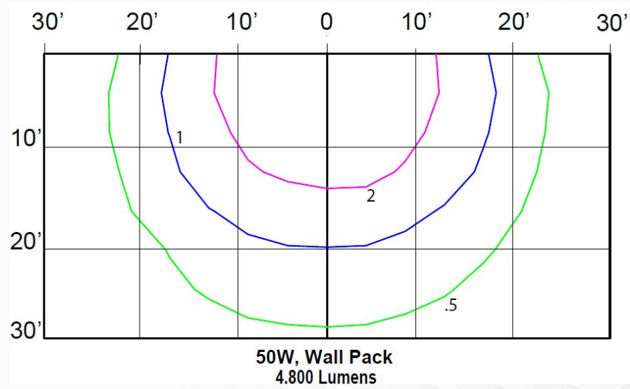
Traditional WP B1-U4-G3 20% of light wasted
