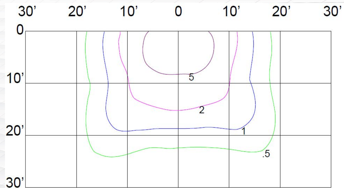
55W, Type IV 6,000 Lumens 15' Mounting Height
