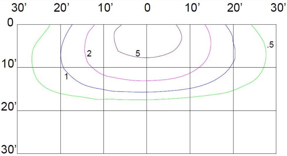
55W, Type III 6,000 Lumens 15' Mounting Height
