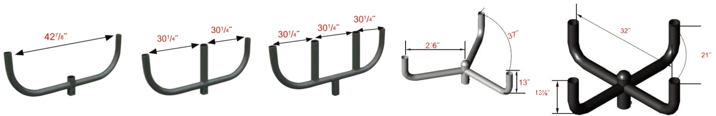
2-3/8" Round Base Bullhorns
