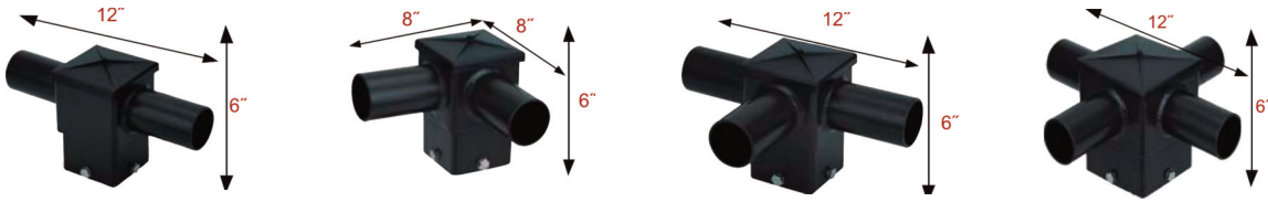
4" Square Horizontal Tenons
