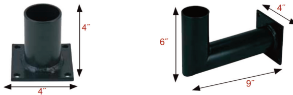
Wall Mount Brackets
